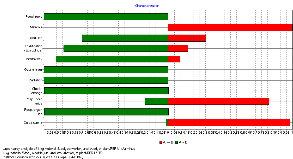
Figure 28 Monte Carlo results of a comparison. In this figure the number of outcomes where converter steel has a higher score than the electro steel are shown per impact category. This allows us to see whether the differences shown in the previous figure are indeed significant. In general we can assume that if 90 to 95% of the Monte Carlo runs are favourable for a product, the difference may be considered significant. Applying this rule means that only the difference between the two processes are not significant for Land use, Acidification and Respiratory inorganic
