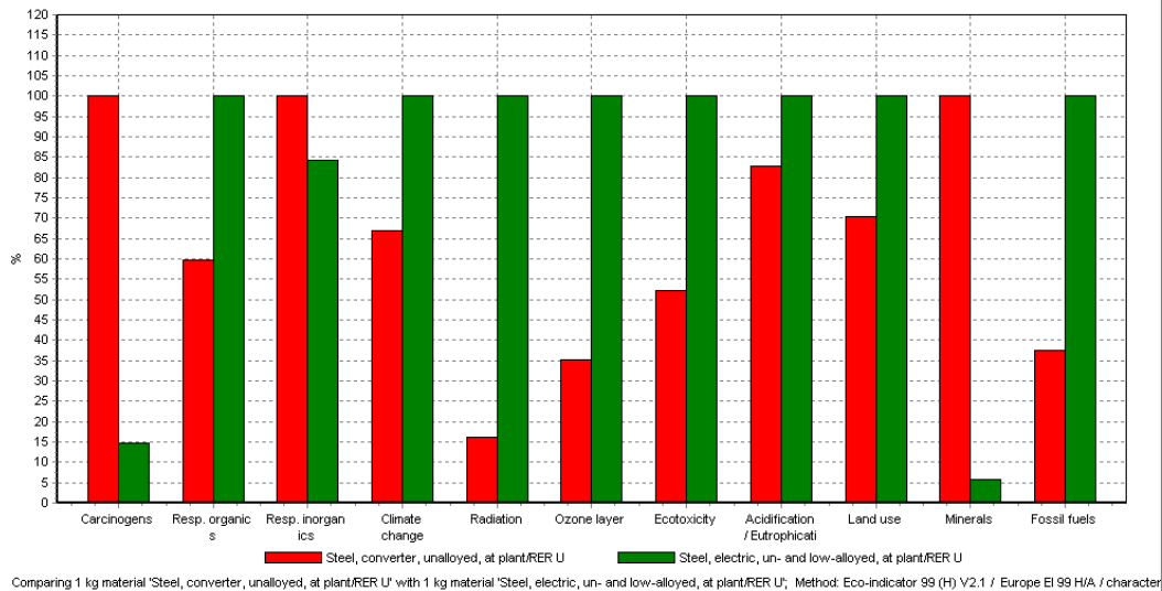
Figure 27 Standard comparison between two ways of producing steel. We see that Electro steel has a lower impact on Carcinogens, Respiratory Inorganic and Minerals
